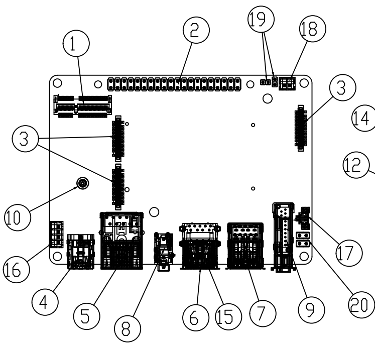
Component top
