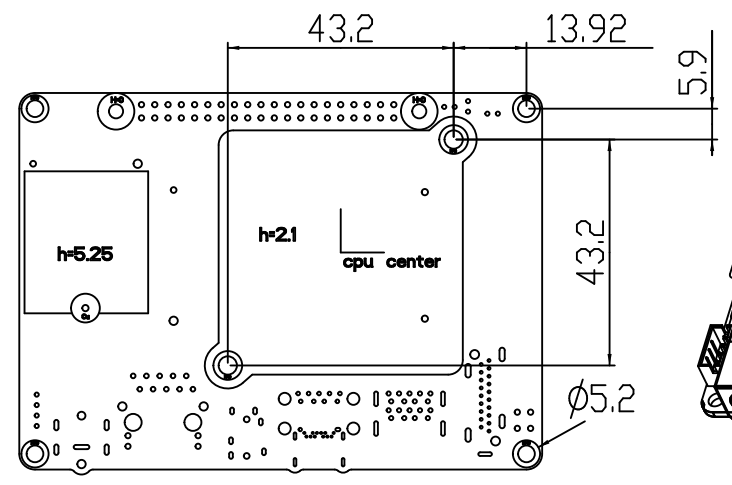
Top limit
